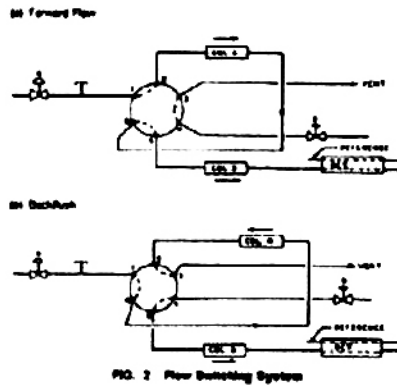
Fig.2 Flow Switching System
