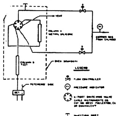
FIG. 1 Tubing Assembly and Instrumentation
